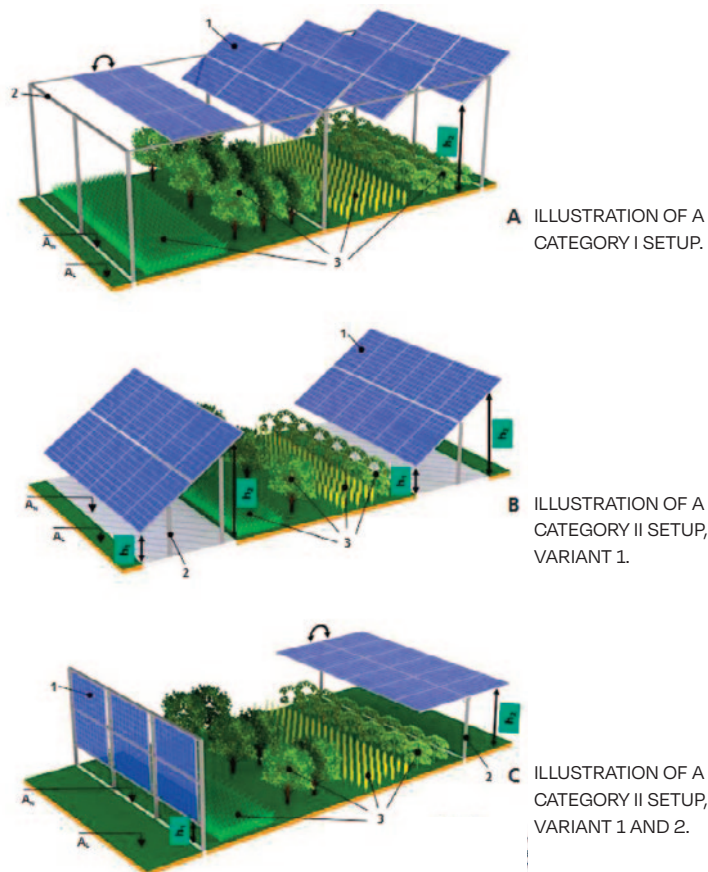
FIGURE 4 DIFFERENT TYPES OF AGRI-PV INSTALLATIONS
